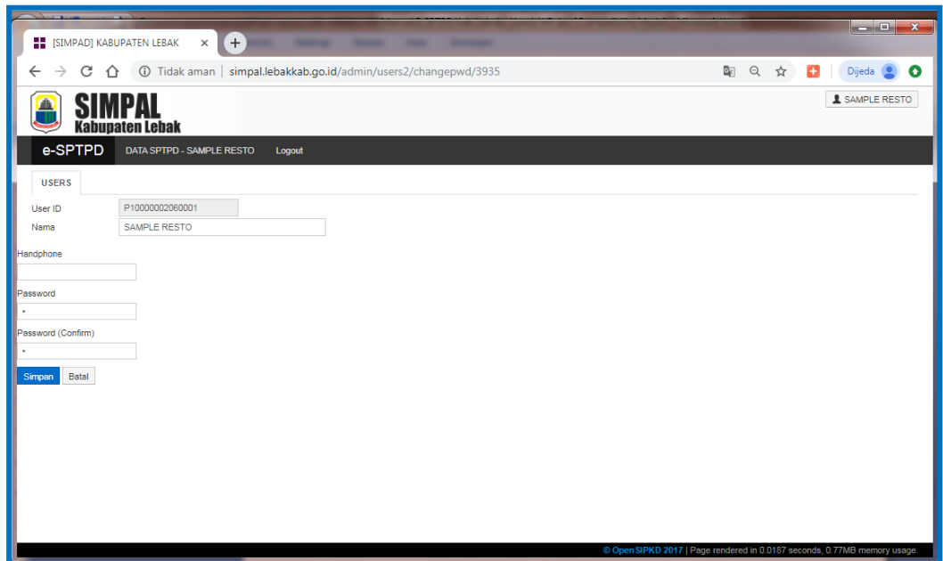
Gambar 9. Ubah Password
